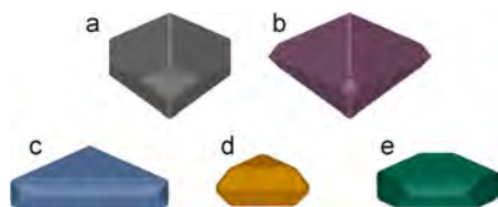
Figure 5. Singly twinned particle shapes obtained by varying the relative surface growth velocities and kinetic growth enhancements. (a) Particle with fast \{111\} growth and no kinetic enhancement, (b) sharp bipyramid obtained with fast \{111\} growth and kinetic enhancement at the re-entrant surfaces, (c) thin triangular platelet obtained with fast \{100\} growth and enhancement at both re-entrant surfaces and twin plane, (d) truncated bitetrahedron obtained with fast \{100\} growth and enhanced growth at the re-entrant surfaces, and (e) thin hexagonal platelet obtained with fast \{100\} growth and enhanced twin growth.
